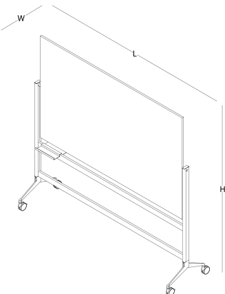
white board W 57 L 155 / 180 H 197
