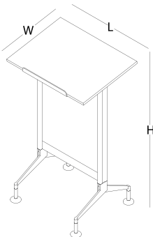
lectern W 57 L 70 H 116
